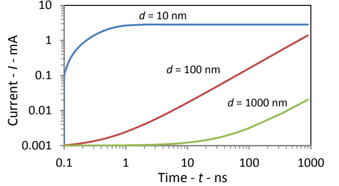
Fig. 4 Transient I – Alq3 Mobility
