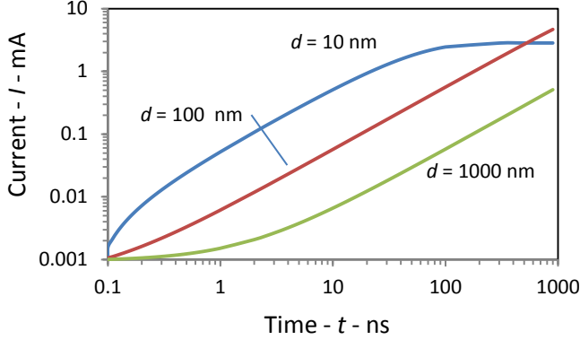
Fig. 6 Transient I – Typical Mobility
