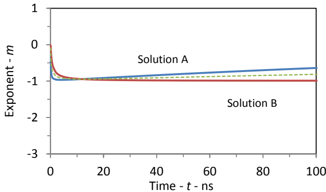
Fig. 8 Transient Exponent m – Typical Mobility
