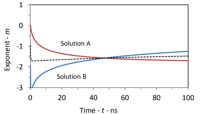
Fig. 5 Transient Exponent m – Alq3 Mobility
