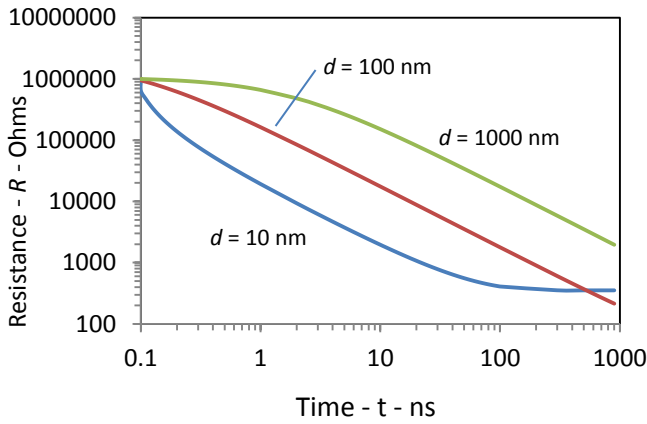
Fig. 7 Transient R – Typical Mobility
