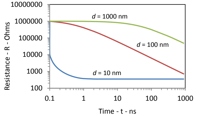
Fig. 5 Transient Resistance R – Alq3 Mobility
