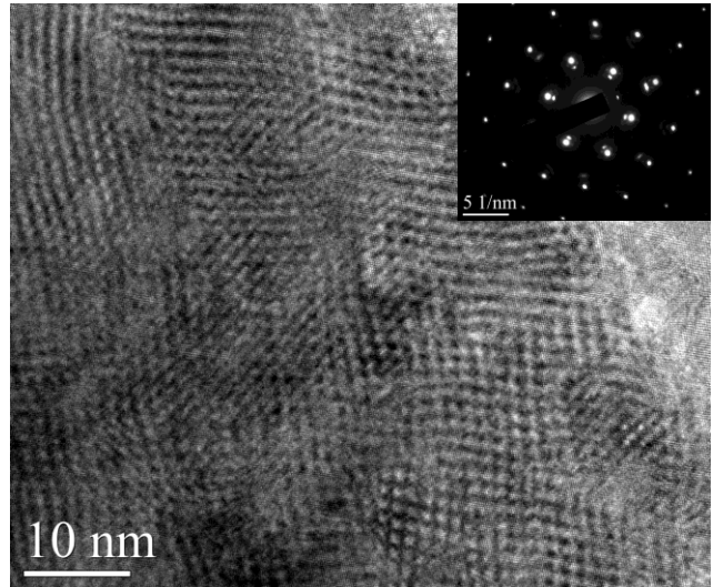
Fig. 3 (110) HRTEM image of a Cu cv 5% sample showing modulation of ~1.6 nm along several crystalline directions. The inset is the diffraction pattern from the area.
