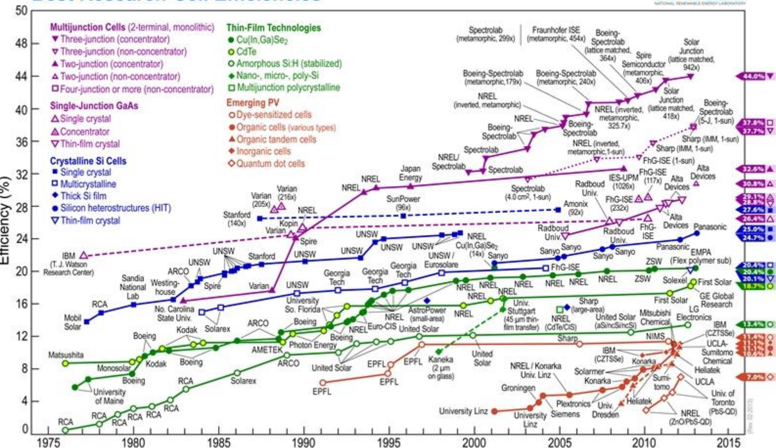
Alta Devices' latest record-breaking cell is the only non-concentrated dual-junction device on NREL's latest chart. The Californian start-up says that its combination of high efficiency and flexibility will be a game-changer in powering mobile devices. Credit: NREL.
